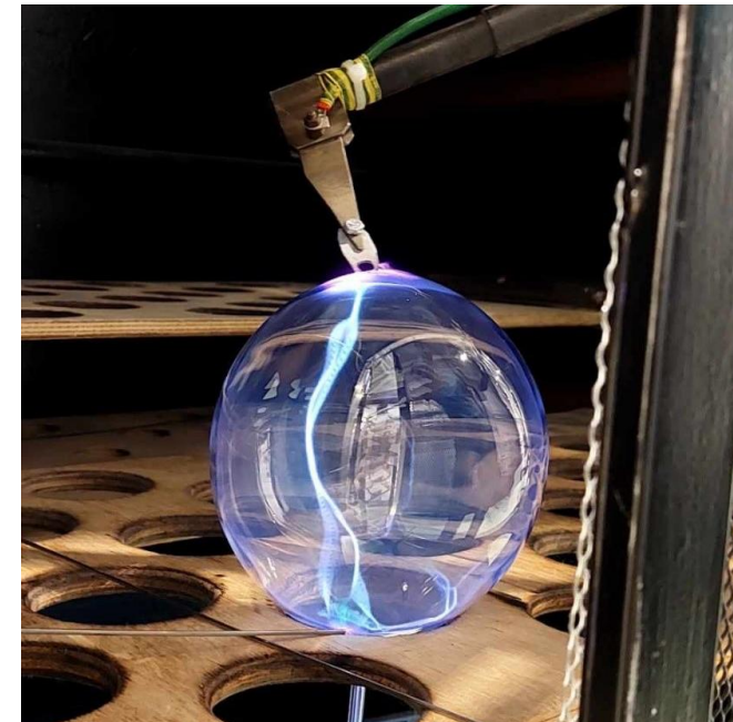
Plasma ignition with a power converter
